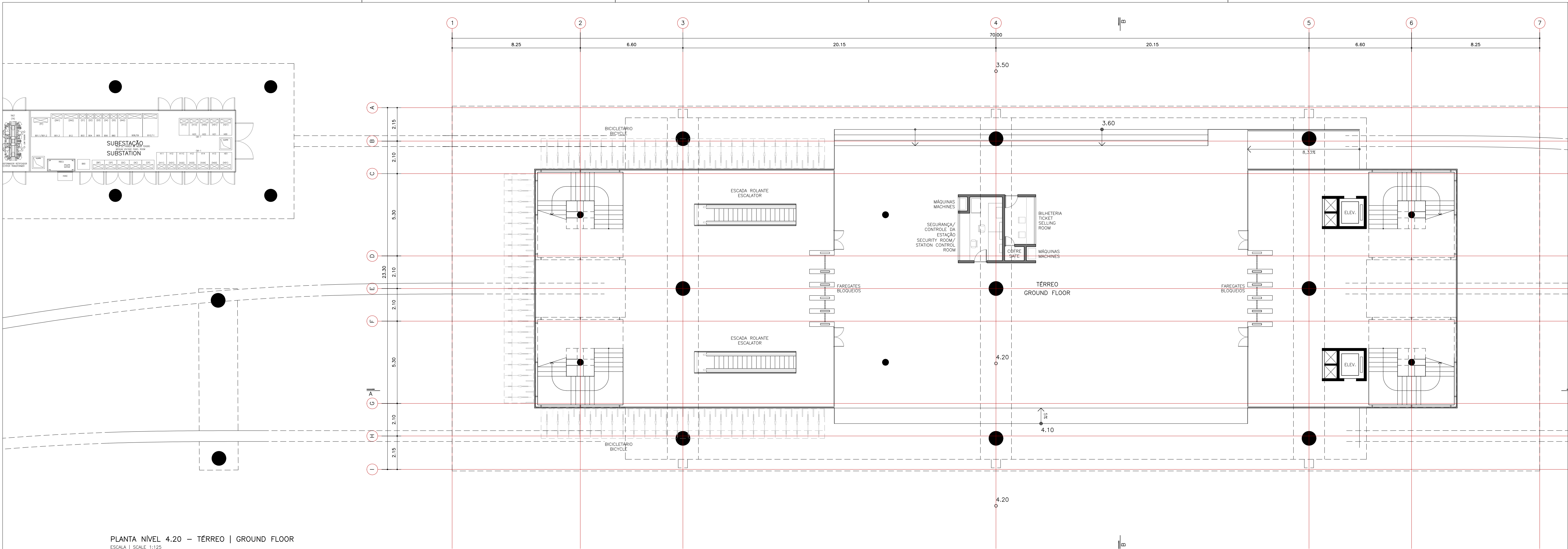
PLANTA NÍVEL 4.20 – TÉRREO | GROUND FLOOR ESCALA | SCALE 1:125
