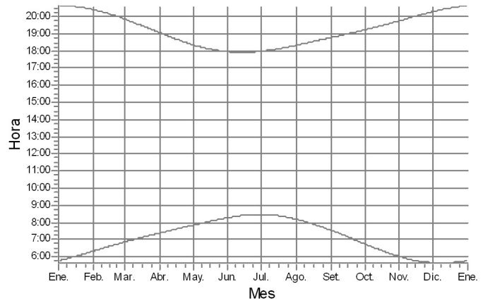
20: GAMESA G114 2650 114.0 !O!hub: 93,0 m (TOT: 150,0 m) (669)
