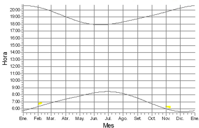
23: GAMESA G114 2650 114.0 !O!hub: 93,0 m (TOT: 150,0 m) (648)
