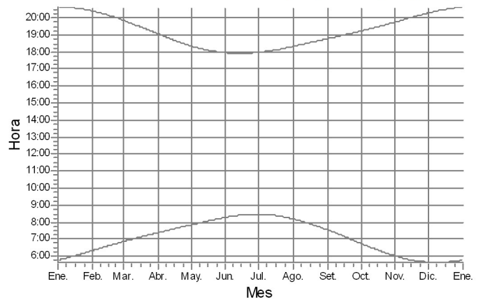
30: GAMESA G114 2650 114.0 !O!hub: 93,0 m (TOT: 150,0 m) (653)
