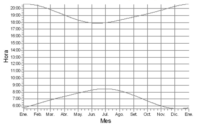
22: GAMESA G114 2650 114.0 !O!hub: 93,0 m (TOT: 150,0 m) (644)
