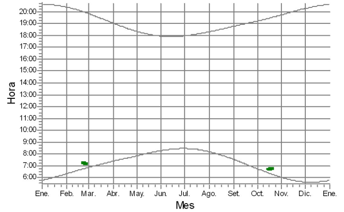
14: GAMESA G114 2650 114.0 !O!hub: 93,0 m (TOT: 150,0 m) (673)
