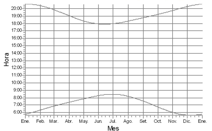
36: GAMESA G114 2650 114.0 !O!hub: 93,0 m (TOT: 150,0 m) (650)
