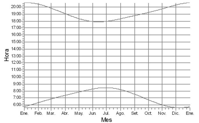
10: GAMESA G114 2650 114.0 !O!hub: 93,0 m (TOT: 150,0 m) (647)
