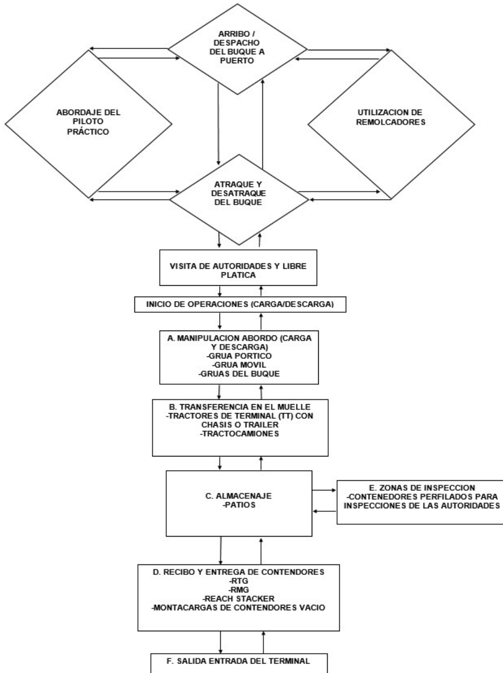
Figure Num. 3.36. Flowchart of operation of containers.
