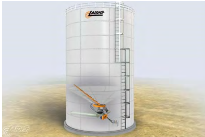
Figure Num. 3.39. Laiding type discharge system. Source: EDIAGRO, 05/2014.
