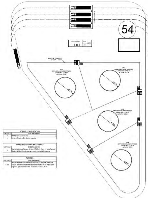
Figure Num. 3.32. Liquid bulk silos. Source: PIO SAS, September 2015.
