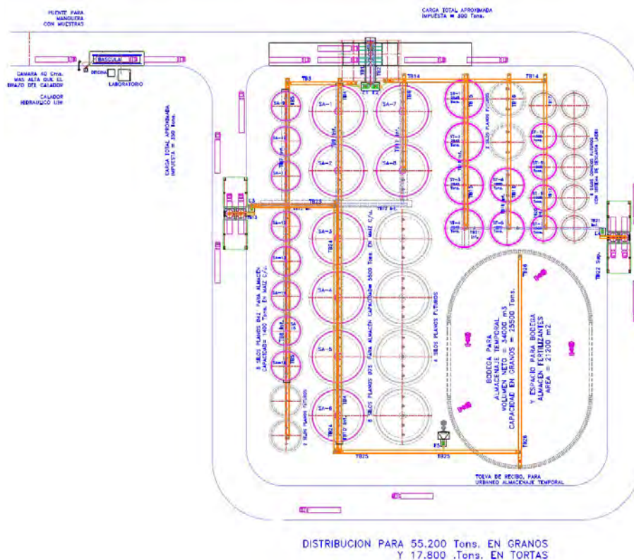
Figure Num. 3.31. Silos and grain storage warehouses Puerto Bahía Colombia de Urabá. Source: EDIAGRO, 2014
