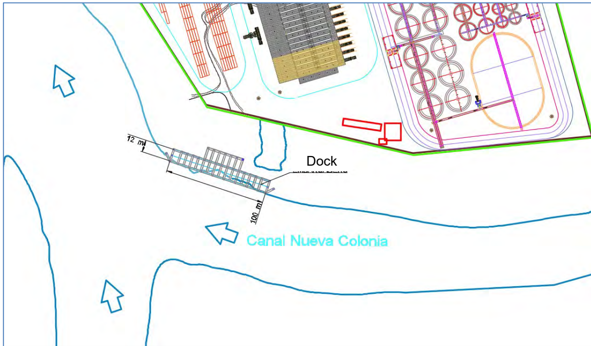
Figure Num. 3.14. Dock on the north shore of the artificial Channel of Nueva Colonia. PIO SAS Sources, September 2015.
