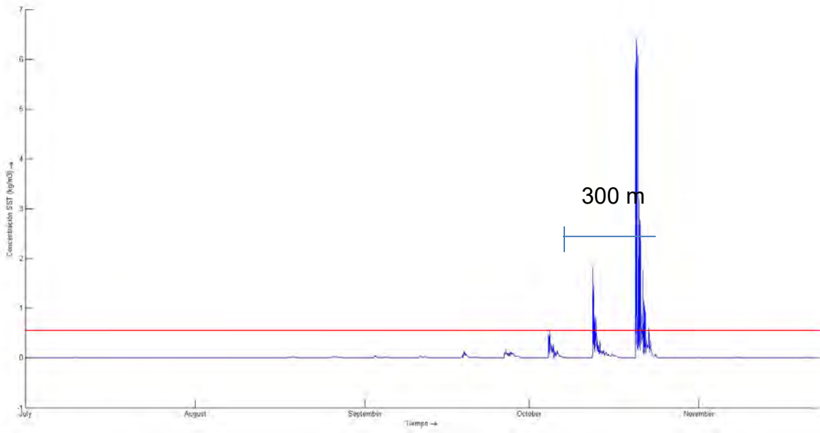
Figure Num. 3.62. Temporary series of material poured into the dump. Source: Aqua & Terra Consultores Asociados
