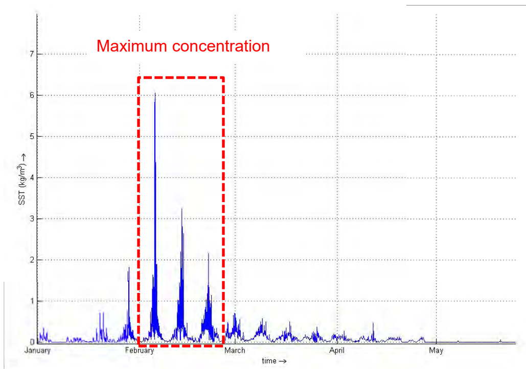
Figure Num. 3.54. Concentration of suspended solids for a discharge cell in the dump Source: Aqua & Terra Consultores Asociados, 2015
