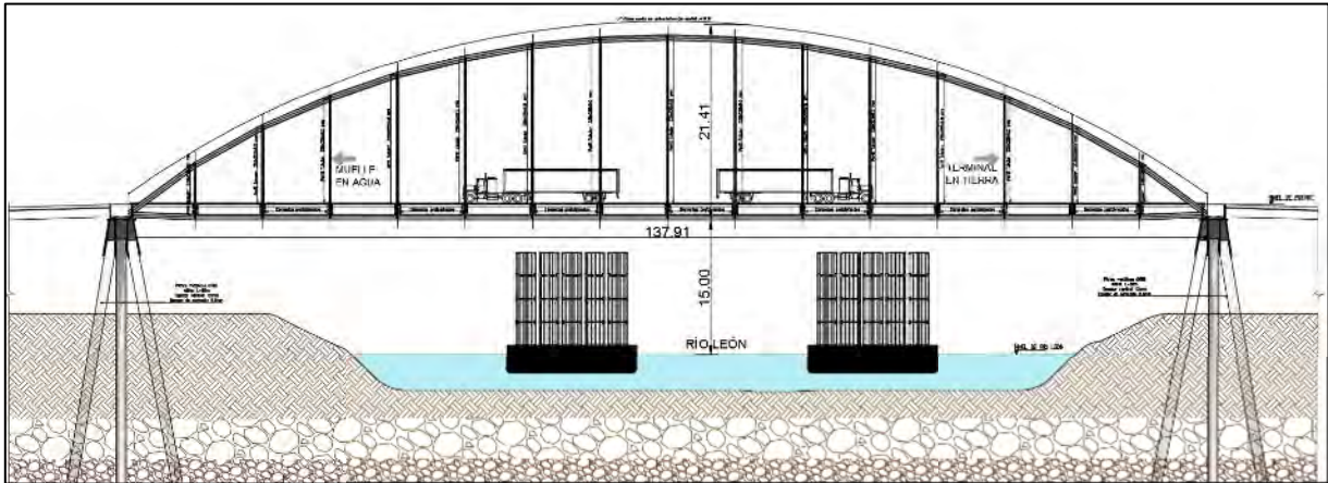
Figure Num. 3.13. Bridge over The León Riiver PIO SAS Sources, September 2015.
