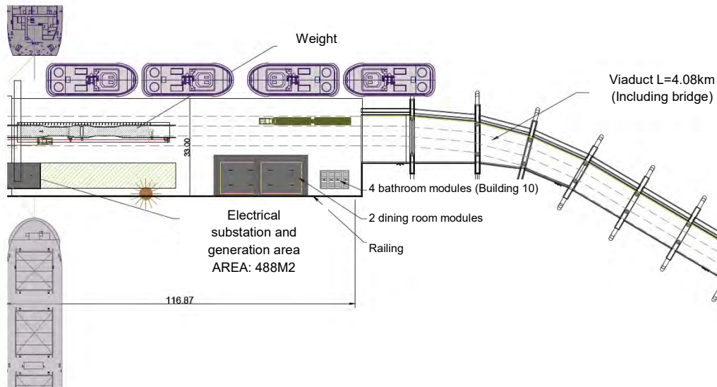
Figure Num. 3.11. Splice platform. Sources: PIO SAS, September 2015.
