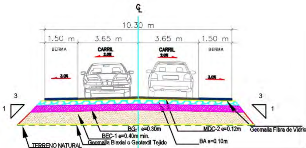
Figure Num. 3.34. Typical section of road structure from Nueva Colonia to Puerto Bahía Colombia de Urabá.
