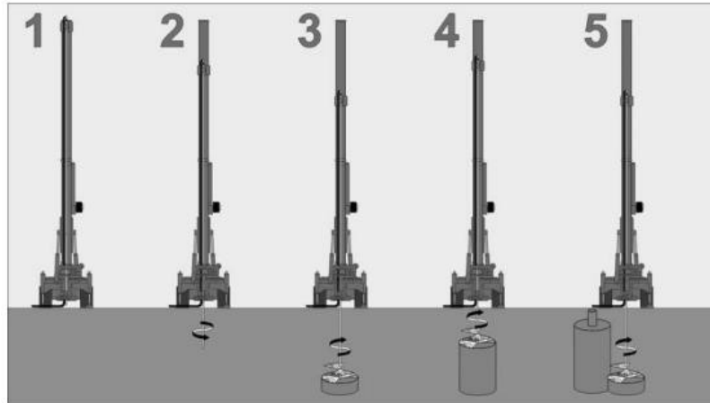
Figure Num. 3.22. Stabilization with jet-grouting Source: Edifica, Geotechnical Study, June 2015.
