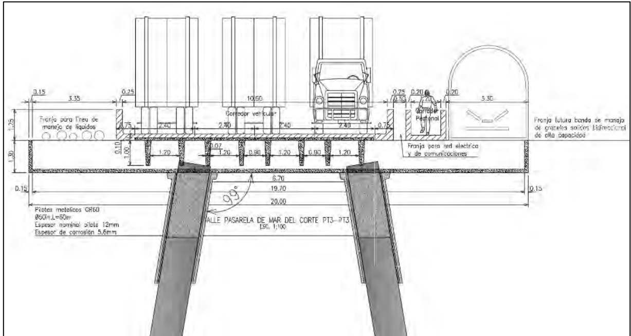
Figure Num. 3.12. Section of the viaduct PIO SAS Sources, September 2015.
