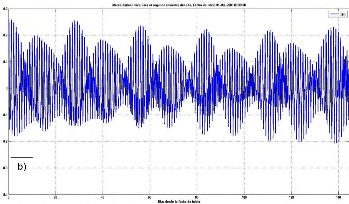
Figure Num. 3.51. Series of astronomical tide for the point to the outskirts of the Golfo de Urabá. a) Series for the first semester of the year and b) series for the second semester of the year.
