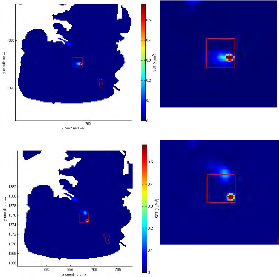
Figure Num. 3.56. Sequence of greater dispersion on the perimeter of the dump. Source: Aqua & Terra Consultores Asociados, 2015
