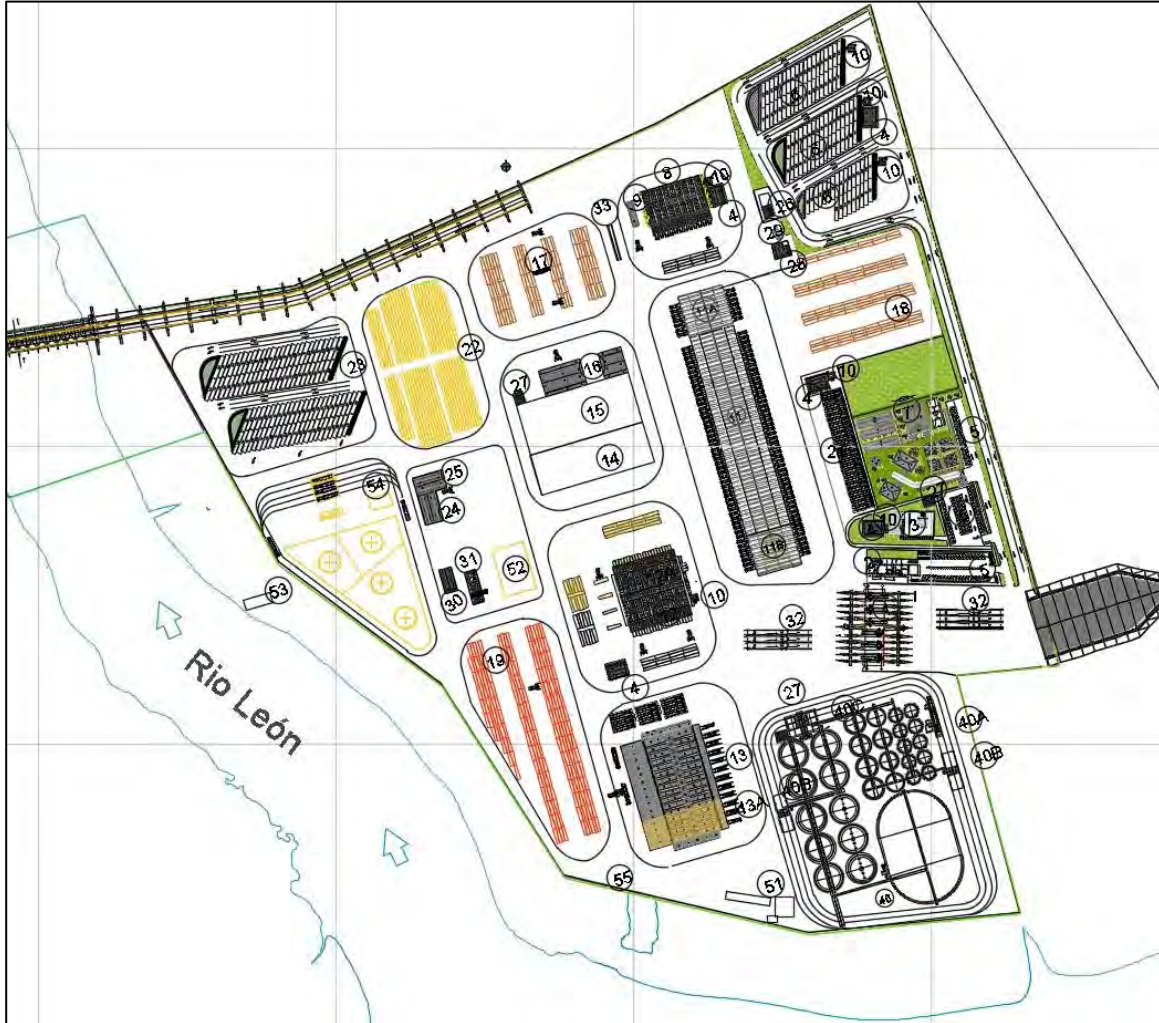
Figure Num. 3.15. Onshore Terminal. PIO SAS Sources, September 2015.
