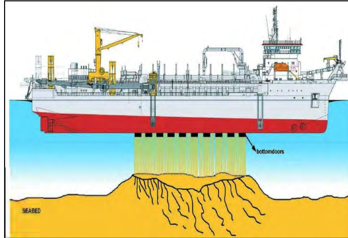
Figure Num. 3.19. The method of unloading dredged material in dump.
