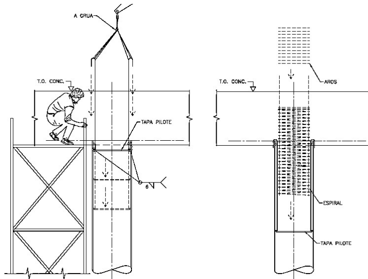
Figure Num. 3.26. Reinforcement installation inside the pile Source: DC-PORT, November 2014.
