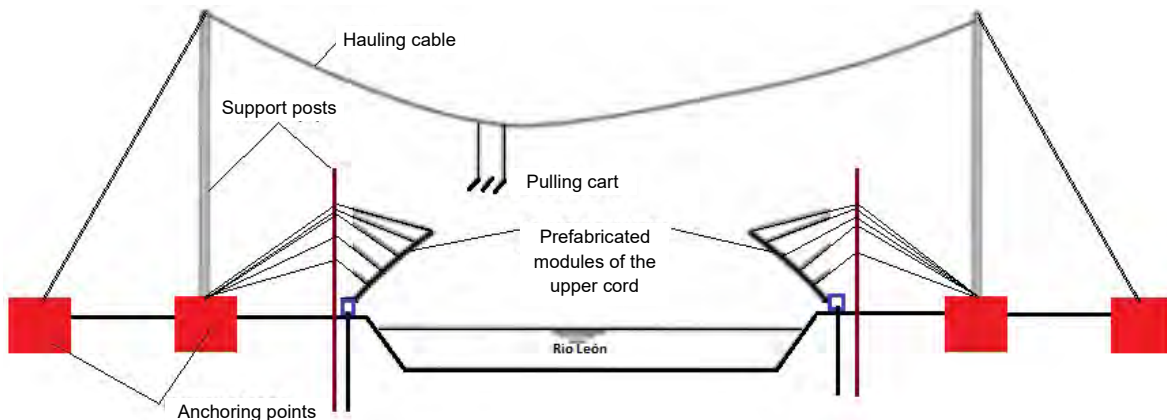
Figure Num. 3.29. Longitudinal elevation assembly of elements that make up the arch Source: DC-PORT, November 2014.
