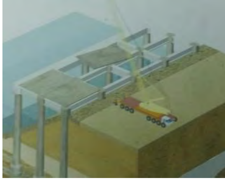
g. Installation of prefabricated slabs
