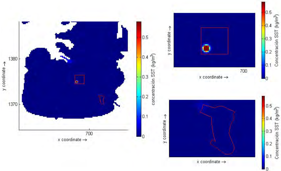
Figure Num. 3.55. Location of dredging area and dump Source: Aqua & Terra Consultores Asociados, 2015
