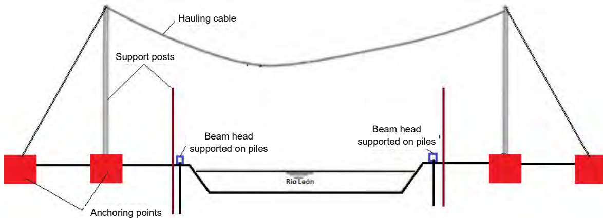
Figure Num. 3.28. Longitudinal elevation support structure and arc starting Source: DC-PORT, November 2014.
