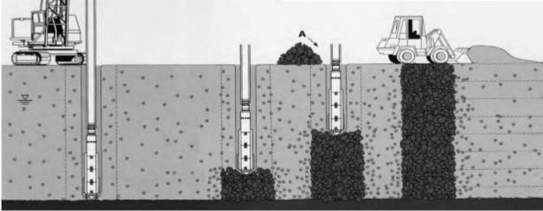
Figure Num. 3.20. Stabilization by gravel columns
