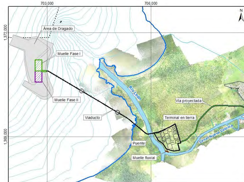
Figure Num. 3.1 Project localization. Source: Aqua & Terra Consultores Asociados.
