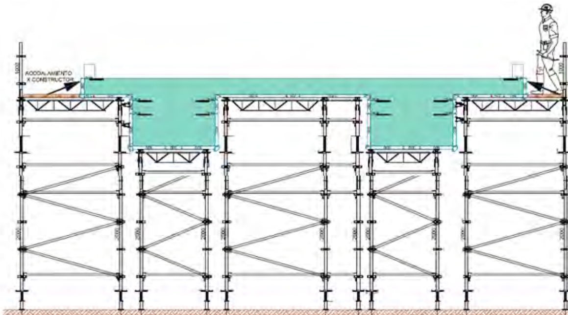
Figure Num. 3.27. Formwork elevation for cast Source: DC-PORT, November 2014.
