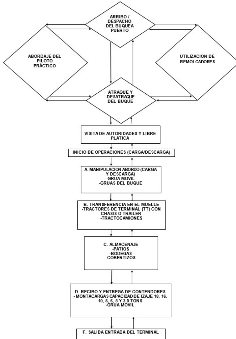
Figure Num. 3.40. Flow diagram of general cargo operation. Source: PIO SAS, October 2015.
