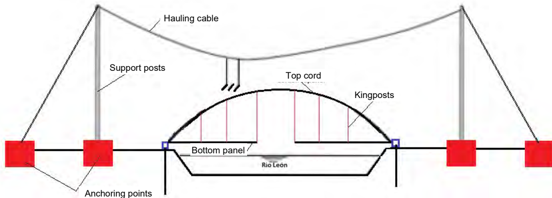
Figure Num. 3.30. Longitudinal elevation assembly of kingposts and lower board Source: DC-PORT, November de 2014.
