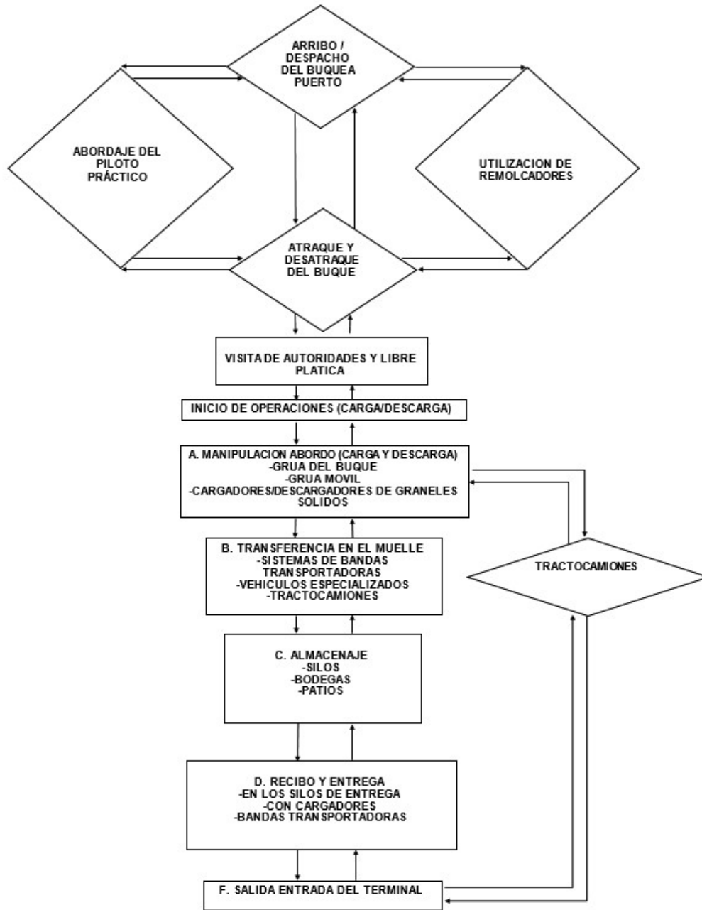
Figure Num. 3.38. Solid bulk operation Flow Chart. Source: PIO SAS, October 2015.
