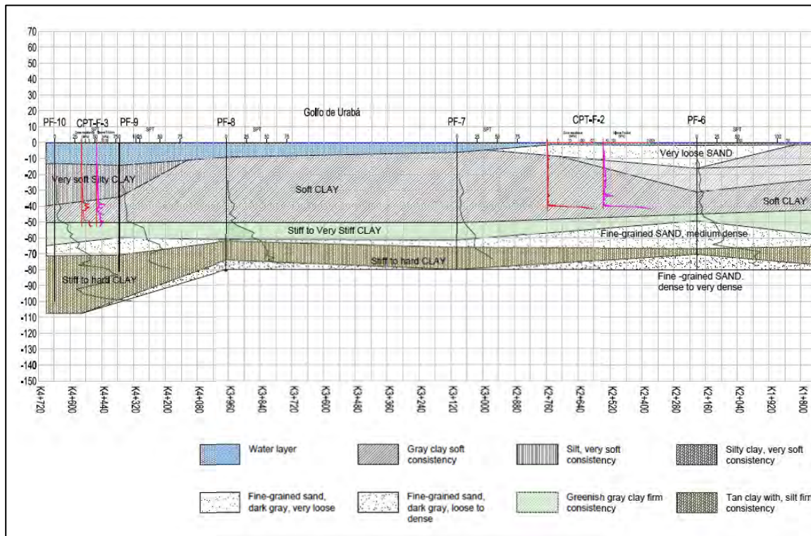
Figure Num. 3.17. Geotechnical drilling and stratigraphic profile. Source: Edifica, Geotechnical Study, June 2015.
