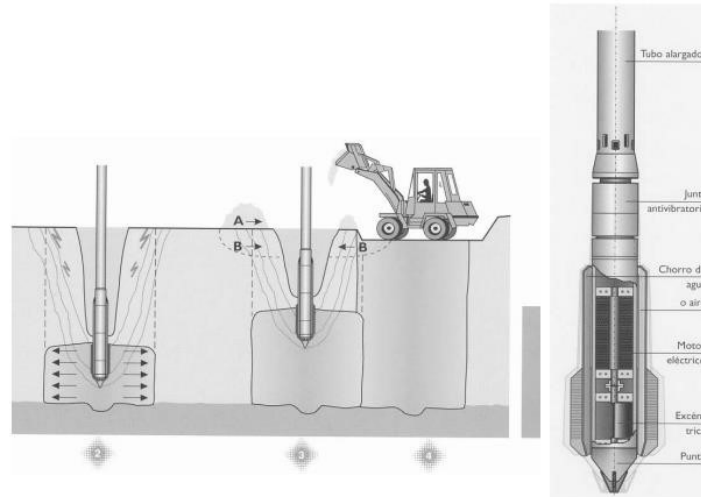
Figure Num. 3.21. Stabilization by vibrocompaction Source: Edifica, Geotechnical Study, June 2015
