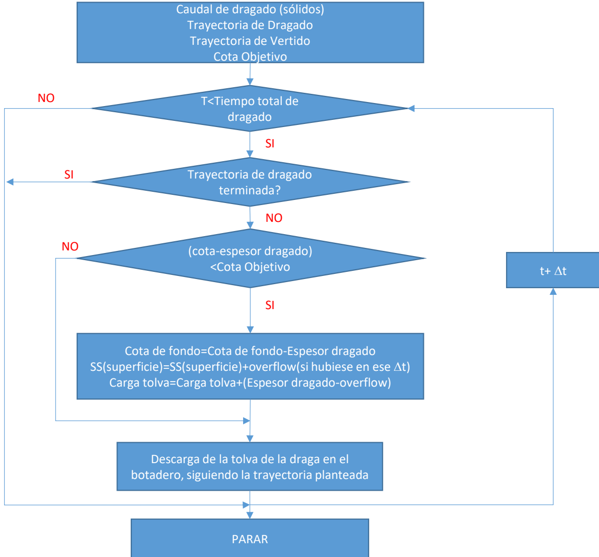
Figure Num. 3.49. Operation diagram of the IH-Dredge methodology (modified by Aqua & Terra Consultores S.A.S) for the simulation of a real-time dredging process with a suction dredger. Source: Aqua&Terra Consultores Asociados S.A.S, 2015.
