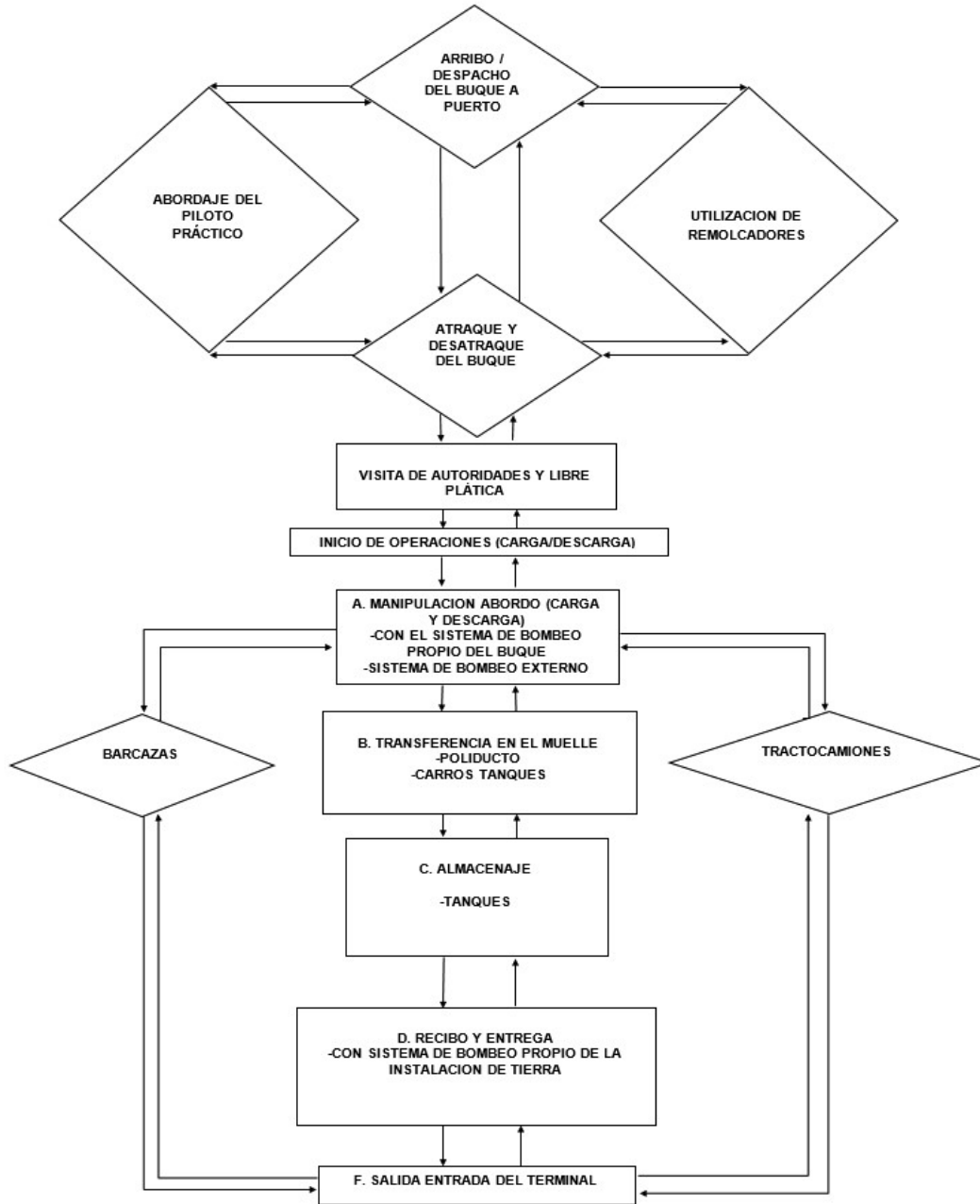
Figure Num. 3.42. Liquid bulk operation flux chart. Source: PIO SAS, October 2015.
