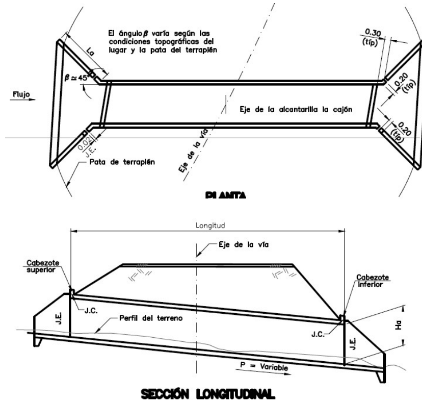
Figure Num. 3.35. Typical section of box culvert Puerto Bahía Colombia de Urabá.
